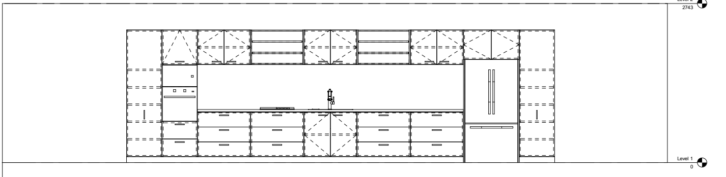
② South 1 : 20
